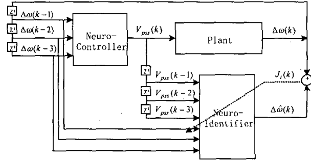
Fig. 9. Training process of the neuro-identifier
