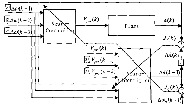
Fig. 5. Structure of the indirect neural network controller
