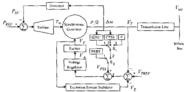
Fig. 1. System model configuration
