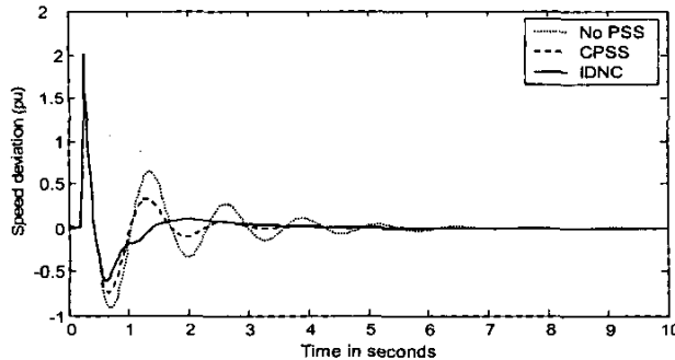
Fig. 11. System response to a three phase short circuit fault ( P=0.401pu, Q=0.017pu ).
