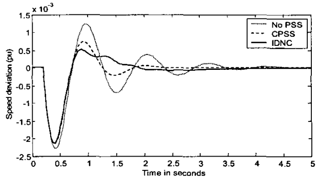
Fig. 13. System response to a simulated transmission line fault ( P=0.401pu, Q=0.017pu ).
