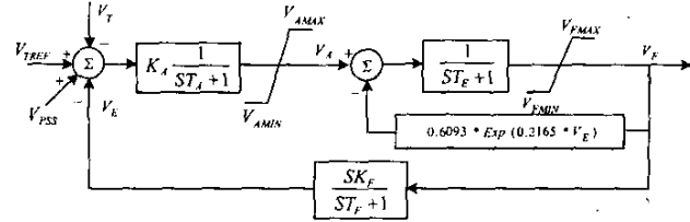
Fig. 3. Block diagram of the excitation system
